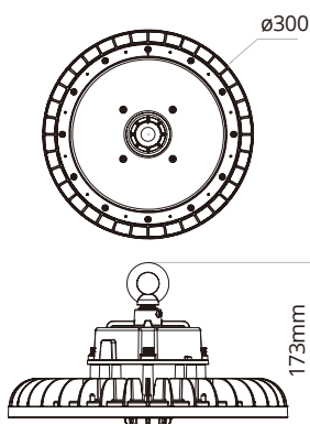
SKYLUX120W-G2
